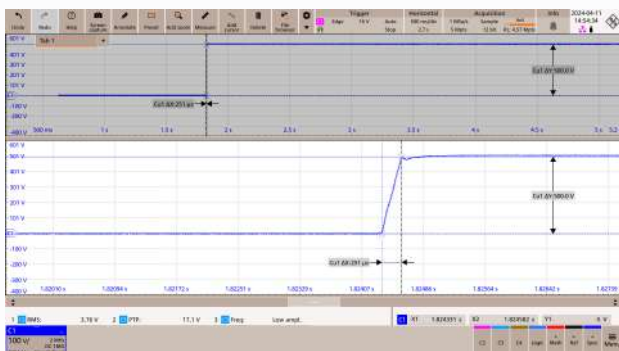
Dynamic response time : 251µs
